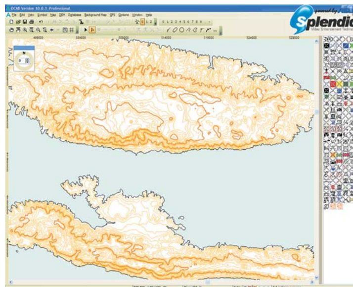
Fig. 6. Contour lines are obtained after several minutes (90m resolution of the elevation point grid)
